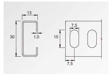
Telex rail
